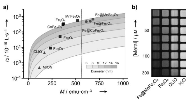
Figure 3. Characterization of transverse relaxivity. a) The transverse relaxivity ( r 2 ) of various MNPs was measured at the fixed Larmor frequency ( f 0 = 20 MHz; B 0 = 0.47 T) and mapped as a function of both the particle size ( d ) and the magnetization ( M ) at 0.47 T. Solid lines are calculated using the outer-sphere theory. The r 2 values of ferrite MNPs increased with larger d and M (squares), but were bounded by the intrinsic M of the material (dotted line for bulk MnFe 2 O 4 ). Because of their stronger magnetization, Fe@MnFe 2 O 4 MNPs passed the boundary and attained higher r 2 relaxivities, with Fe@MnFe 2 O 4 assuming the highest value. b) Phantom images ( f 0 = 300 MHz; B 0 = 7 T) further verified the superiority of Fe@MnFe 2 O 4 MNPs as imaging agents in MRI. CLIO, cross-linked iron oxide nanoparticle; MION, monocrystalline iron oxide nanoparticle.
