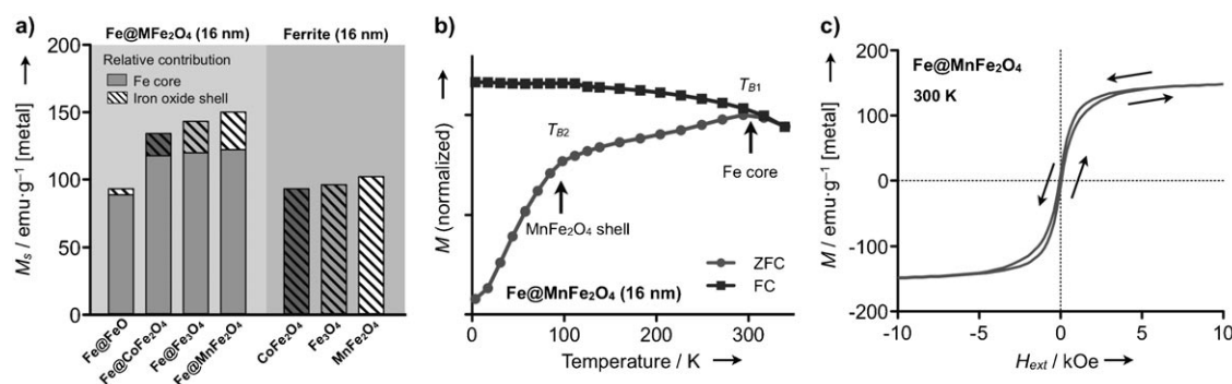
Figure 2. Magnetic properties of Fe@ferrite MNPs. a) All Fe@MnFe 2 O 4 MNPs ( d = 16 nm) had higher M s than similarly sized ferrite MNPs. Among the Fe@MnFe 2 O 4 MNPs, the overall M s was within the same order of magnitude as the shell magnetization. b) Temperature-dependent magnetization curves of Fe@MnFe 2 O 4 MNPs showed distinct peaks at two different temperatures, T B1 and T B2 , indicating separate onset of superparamagnetism in the core ( T B1 ) and the shell ( T B2 ). c) The field-dependent magnetization ( M ) of Fe@MnFe 2 O 4 MNPs at 300 K showed an unusual feature for MNPs: negligible remanent moments but the presence of hysteresis. ZFC, zero-field cooling; FC, field-cooling.
